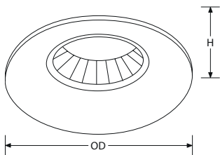
AA-DLM370 (H) 48mm Height (OD) 85mm Overall (Ø) (CO) 76mm Cutout (Ø)
