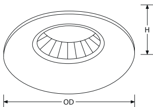
AA-DLM360 (H) 32mm Height (OD) 76mm Overall (Ø) (CO) 72mm Cutout (Ø)
