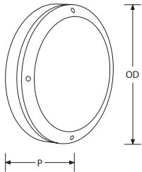
AA-BHD18-CS AA-BHDE18-CS (OD) 277mm Overall Ø (OD) 277mm Overall Ø (P) 80mm Projection (P) 80mm Projection
